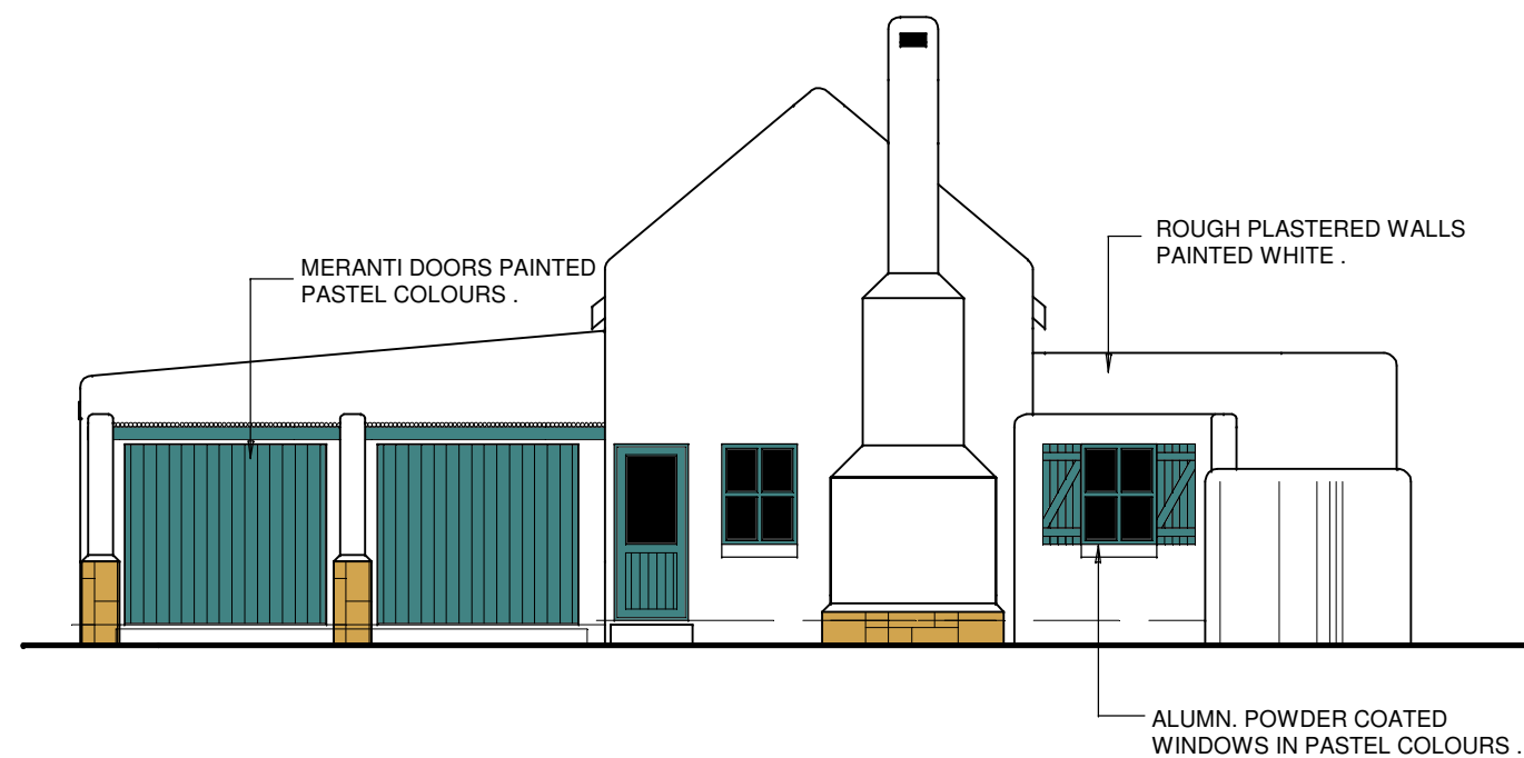
TYPICAL STREET ELEVATION
