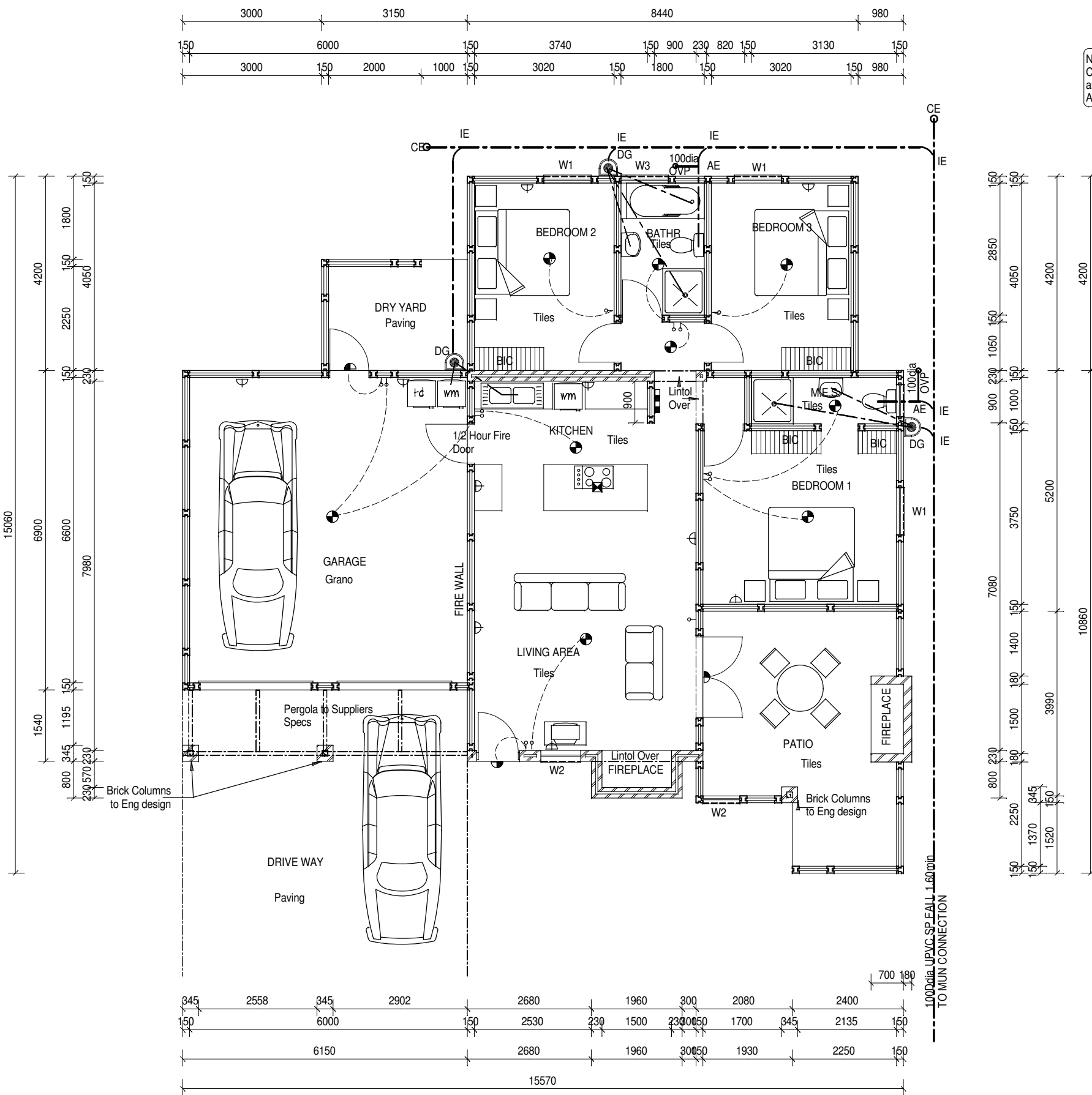
FLOOR LAYOUT Scale 1:100
